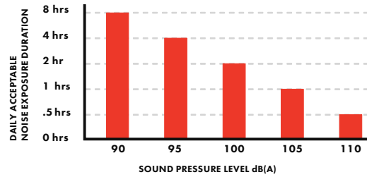
OSHA SAFE NOISE EXPOSURE LIMITS CHART
